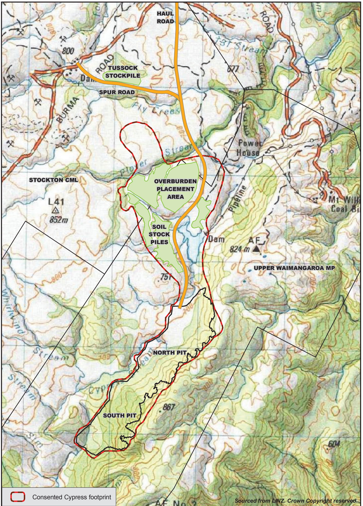
Figure 2.1a: Cypress Mine Revised Layout
